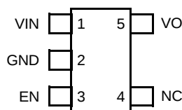
ISL9008 (5 LD SC-70) TOP VIEW
