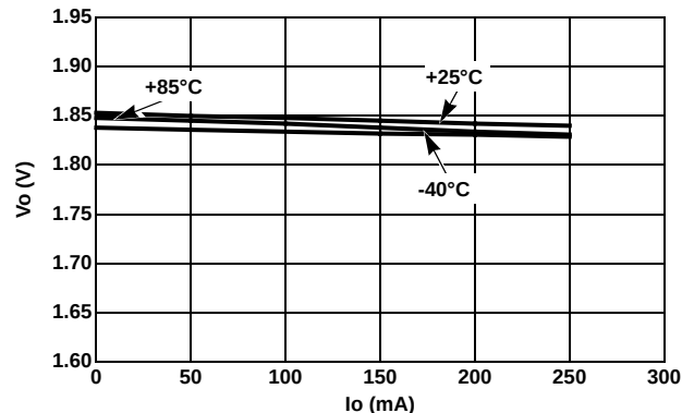
FIGURE 4. LOAD REGULATION vs TEMPERATURE ( V_{OUT} = 1.85V )
