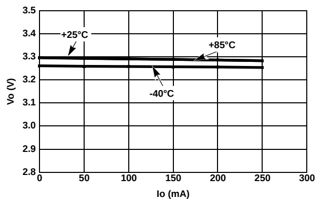
FIGURE 6. LOAD REGULATION vs TEMPERATURE ( V_{OUT} = 3.3V )
