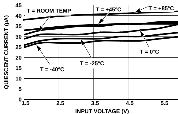
FIGURE 2. QUIESCENT CURRENT vs INPUT VOLTAGE ( V_{OUT} = 1.85V )
