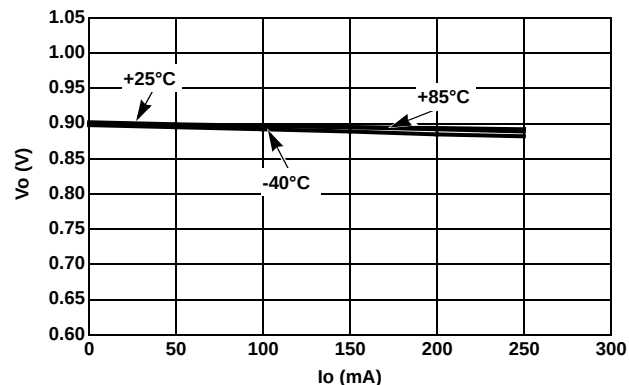
FIGURE 8. LOAD REGULATION vs TEMPERATURE ( V_{OUT} = 0.9V )
