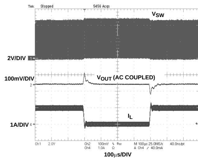
FIGURE 16. LOAD TRANSIENT TEST (MODE = GND, V_{IN} = 5.0V ; V_O = 1.5V ; I_O = 0.01A-1A )
