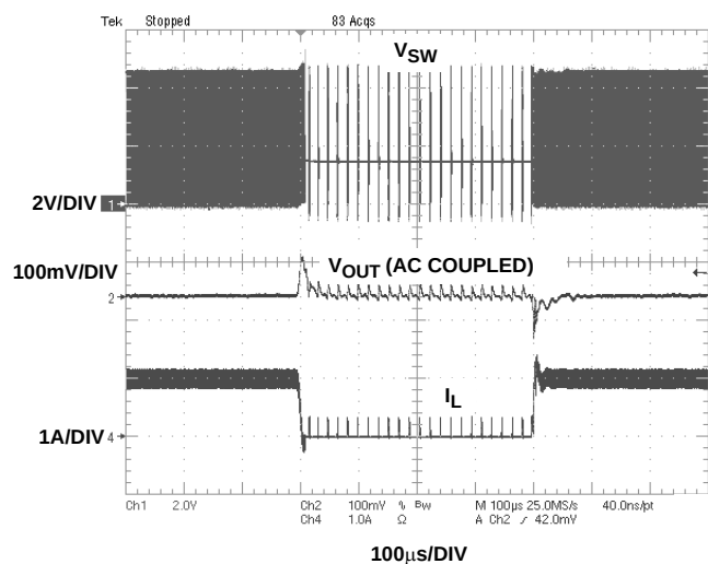
FIGURE 15. LOAD TRANSIENT TEST (MODE = V_{IN} , V_{IN} = 5.0V ; V_O = 1.5V ; I_O = 0.01A-1A )
