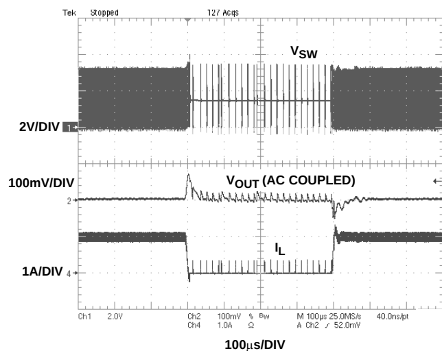
FIGURE 17. LOAD TRANSIENT TEST (MODE = V_{IN} , V_{IN} = 3.6V ; V_O = 1.5V ; I_O = 0.01A-1A )
