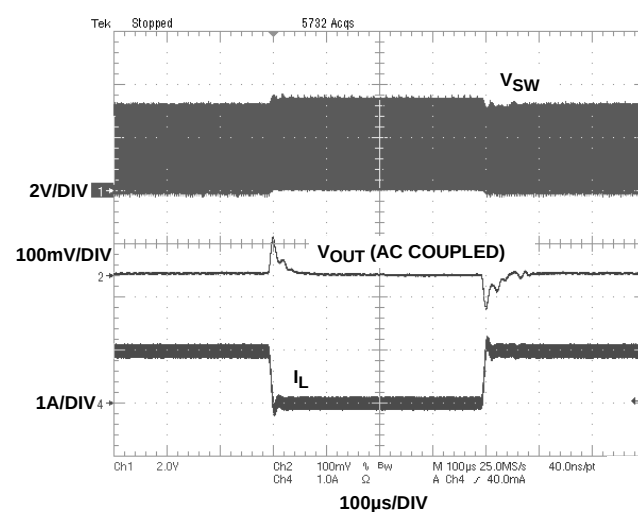
FIGURE 18. LOAD TRANSIENT TEST (MODE = GND, V_{IN} = 3.6V ; V_O = 1.5V ; I_O = 0.01A-1A )
