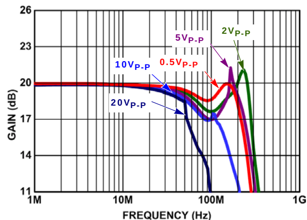
FIGURE 8. LARGE SIGNAL FREQUENCY RESPONSE
