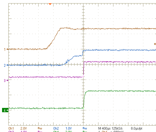
FIGURE 15. 4-CHANNEL DEFAULT START-UP @ FULL LOAD CH1: V0DCD1 (2V/DIV), CH2: V0DCD2 (1V/DIV), CH3: V0LD01 (1V/DIV), CH4: V0LD02 (2V/DIV)
