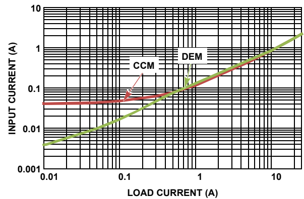
FIGURE 11. PWM1 INPUT CURRENT COMPARISON WITH MODE = CCM/DEM
