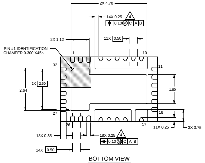
BOTTOM VIEW
