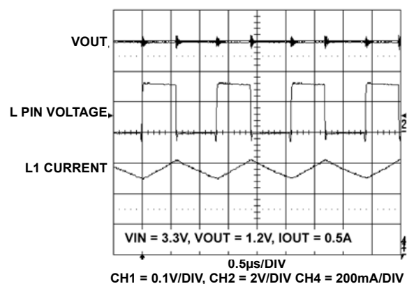
FIGURE 10. SWITCHING WAVEFORM FOR ISL6410
