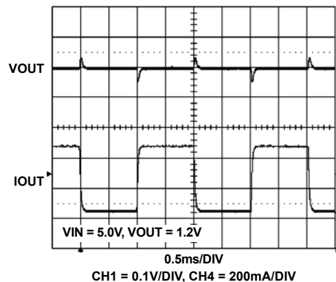
FIGURE 13. TRANSIENT LOAD WAVEFORM FOR ISL6410A
