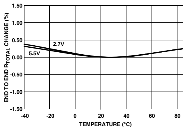
FIGURE 9. END TO END R_{TOTL} % CHANGE vs TEMPERATURE
