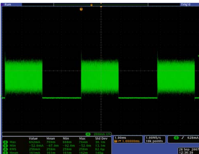
FIGURE 10. IL AT 50% PWM DIMMING
