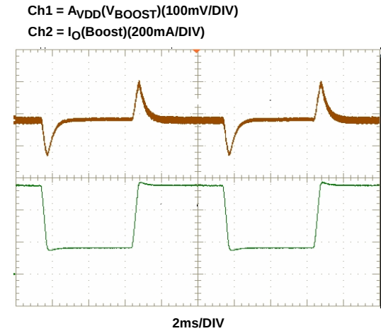
FIGURE 12. TRANSIENT RESPONSE OF BOOST
