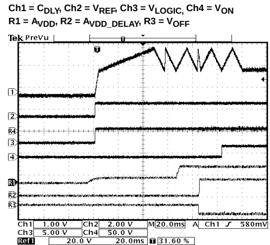
FIGURE 14. START-UP SEQUENCE
