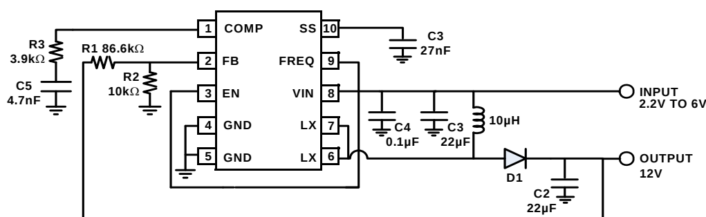
FIGURE 1. TYPICAL APPLICATION CIRCUIT
