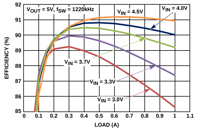
FIGURE 3. V_{OUT} = 5V EFFICIENCY
