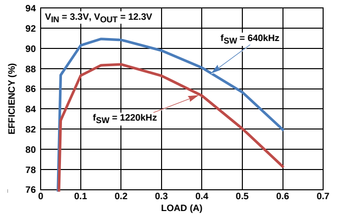
FIGURE 7. V_{OUT} = 12.3V EFFICIENCY
