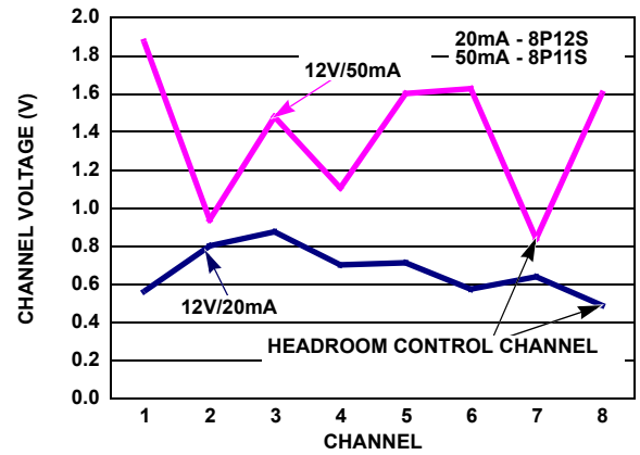
FIGURE 11. TYPICAL CHANNEL VOLTAGE EXAMPLE
