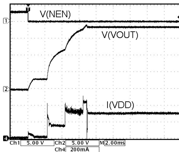
FIGURE 7. START-UP TO 18V @ SEL = 1 (V_{DD} = 3.6V, R_L = 360\Omega)
