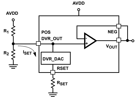
FIGURE 21. DVR_OUTPUT CIRCUIT CONNECTION EXAMPLE
