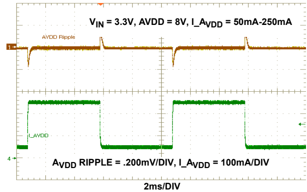
FIGURE 2. AVDD LOAD REGULATION
