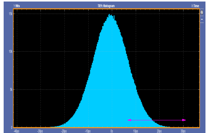
FIGURE 26. SERDES Histogram at 3.0Gbps
