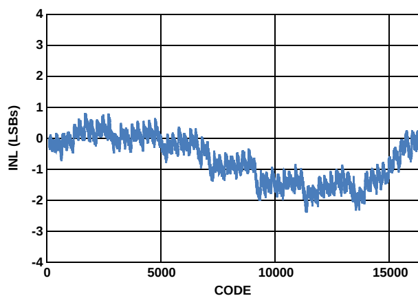
FIGURE 11. INTEGRAL NONLINEARITY
