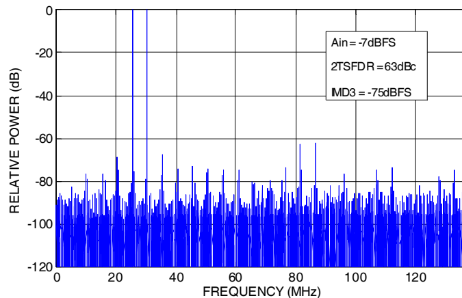
FIGURE 18. TWO-TONE SPECTRUM; f_{IN} = 300MHz, 305MHz
