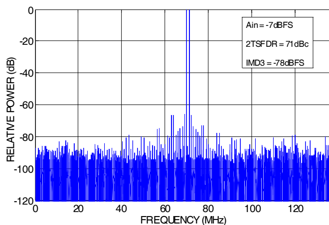
FIGURE 16. TWO-TONE SPECTRUM; f_{IN} = 69MHz, 70MHz
