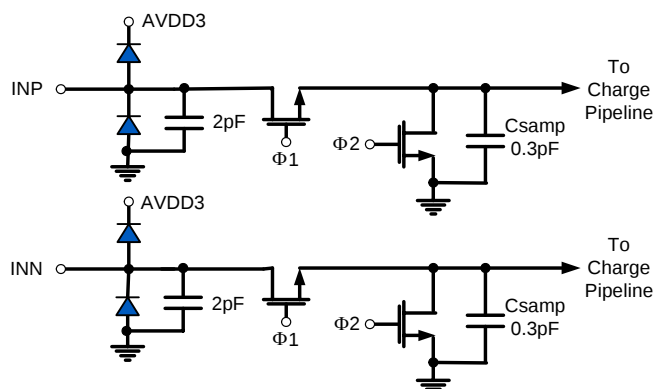
FIGURE 28. ANALOG INPUTS
