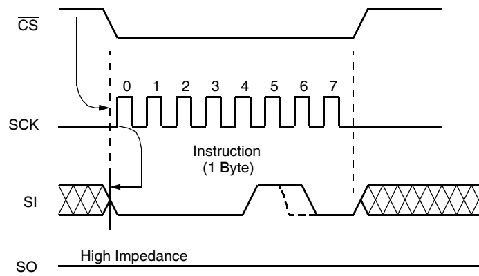
FIGURE 7. WREN/WRDI SEQUENCE
