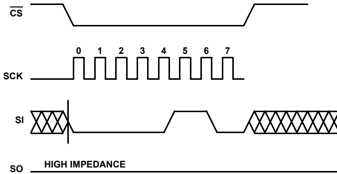
FIGURE 7. WRITE ENABLE LATCH SEQUENCE
