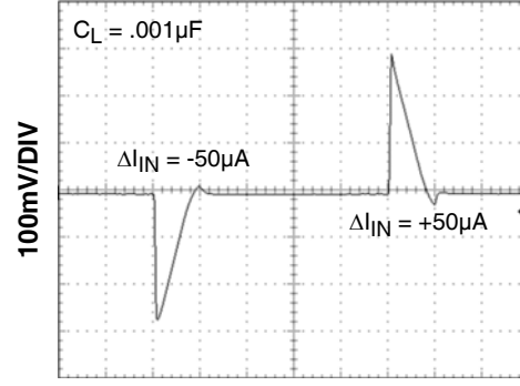
50μA LOAD TRANSIENT RESPONSE
