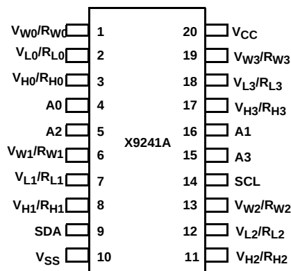
X9241A (20 LD DIP, SOIC, TSSOP) TOP VIEW
