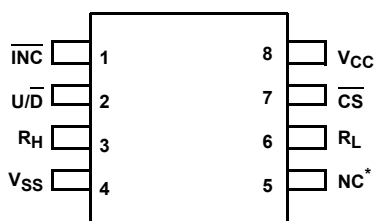
X93154 (8 LD MSOP) TOP VIEW
