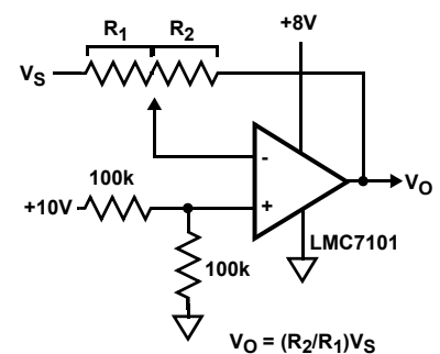
FIGURE 5. SINGLE SUPPLY INVERTING AMPLIFIER
