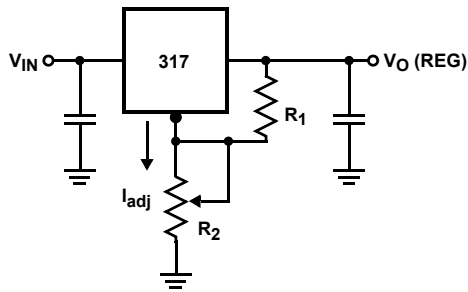
FIGURE 6. VOLTAGE REGULATOR
