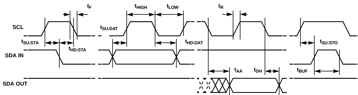
FIGURE 1. BUS TIMING
