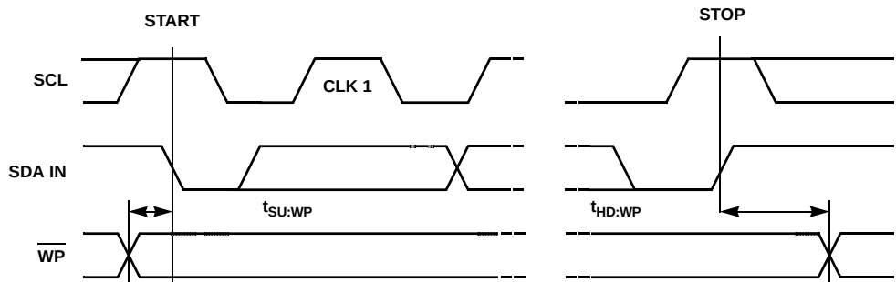
FIGURE 2. WP PIN TIMING
