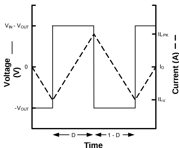
FIGURE 12. INDUCTOR WAVEFORM
