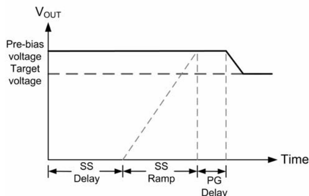
FIGURE 17. OUTPUT RESPONSES TO PRE-BIAS VOLTAGES
