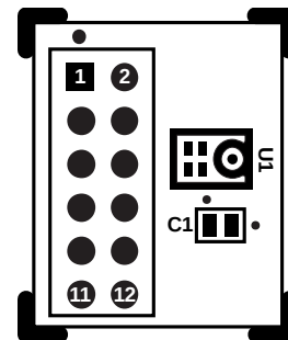
Figure 2. PCB Layout
