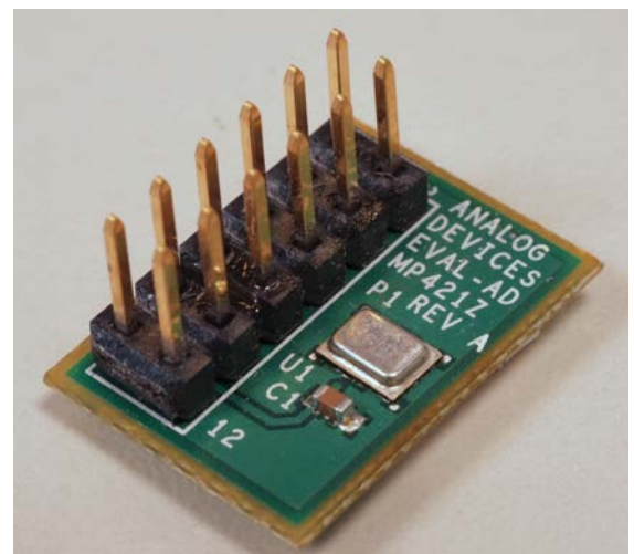
Figure 2. PCB Layout
