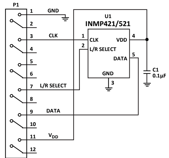
Figure 1. Evaluation Board Schematic
