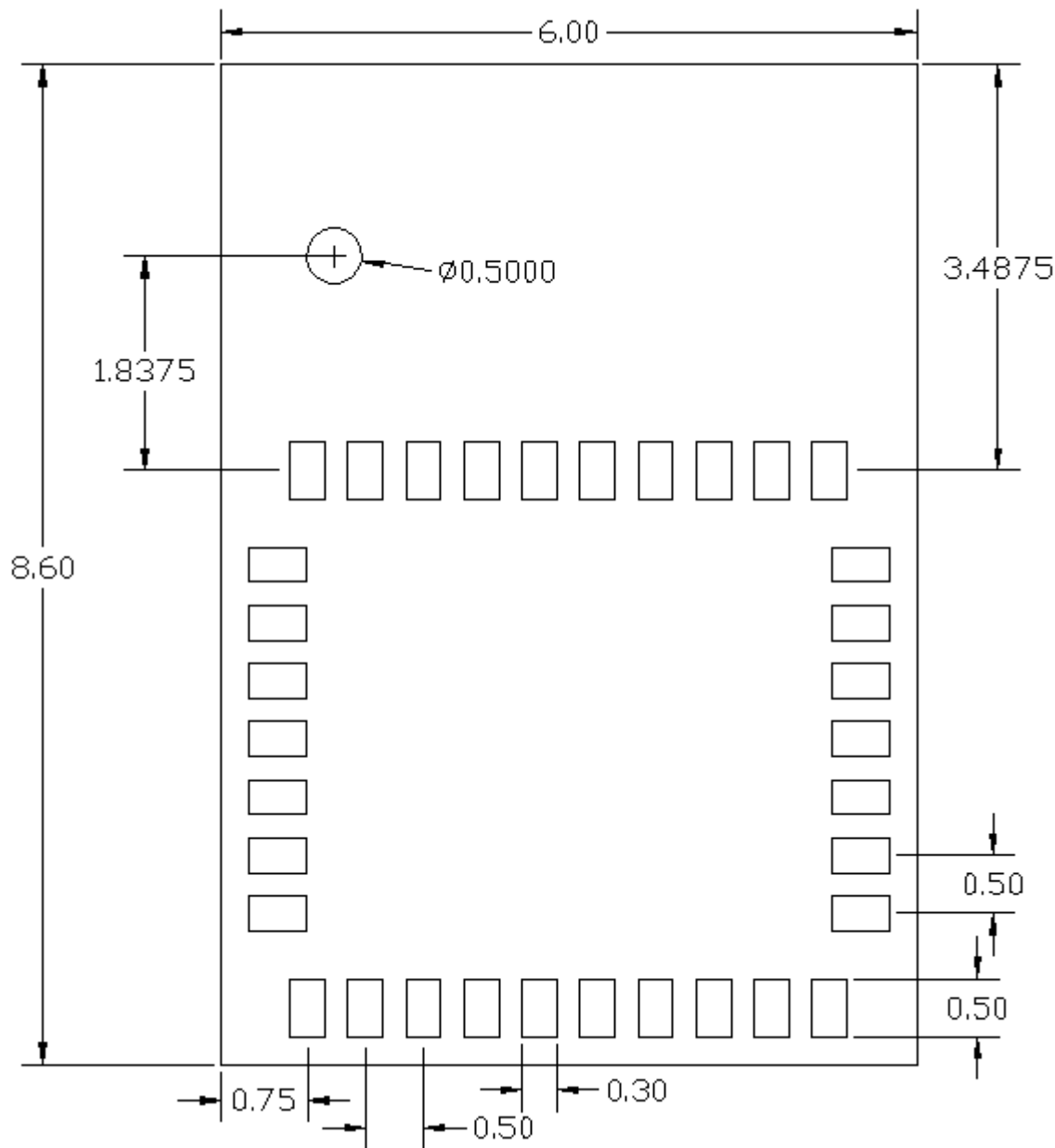
TOP View
