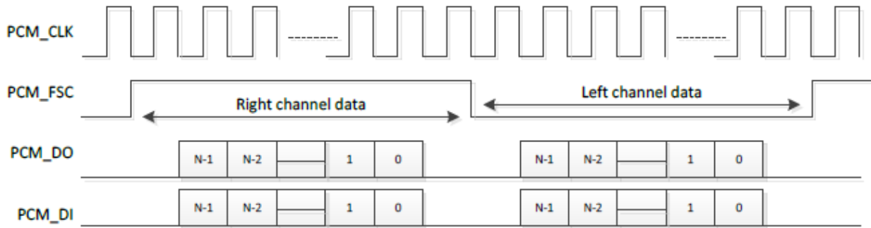
Figure 47 I2S Mode
