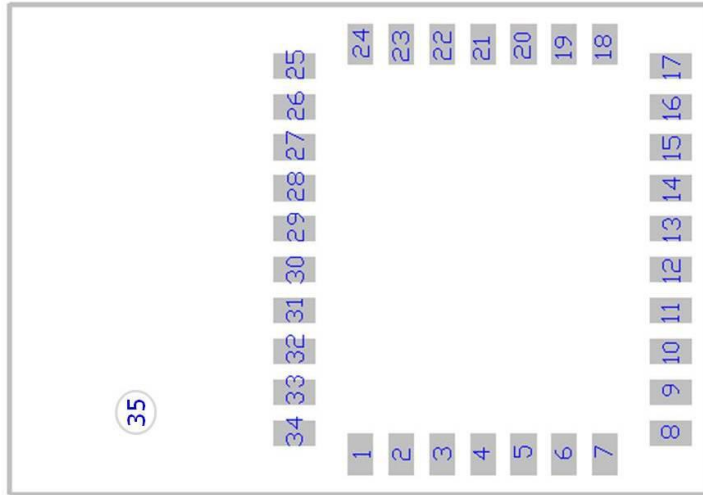
Figure 3. TOP VIEW
