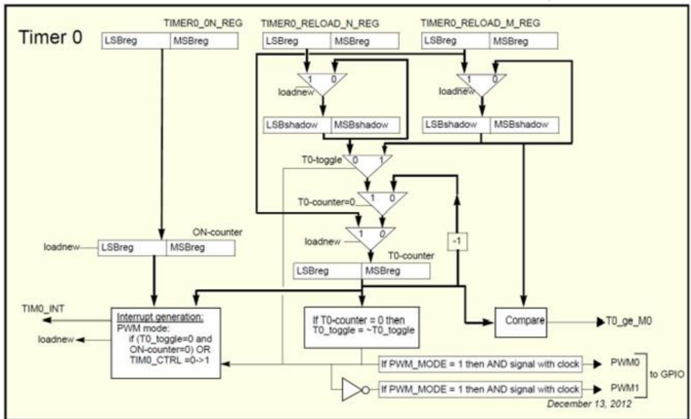
Figure 33 Timer 0 Block Diagram
