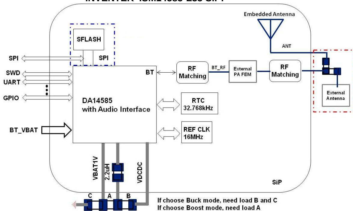
Figure 2 Inventek ISM14585-L35 SiP Block Diagram
