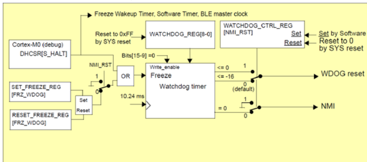
Figure 37 Watchdog Timer Block Diagram
