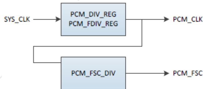
Figure 45 PCM clock generation
