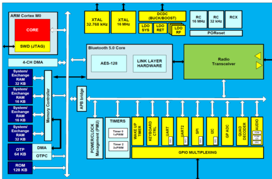
Figure 1 Dialog DA14585 SoC Block Diagram
