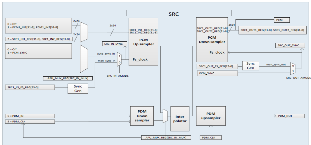
Figure 40 Sample Rate Converter block diagram
