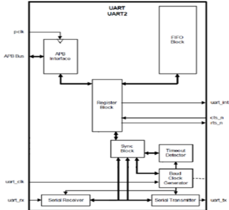
Figure 20 UART Block Diagram
