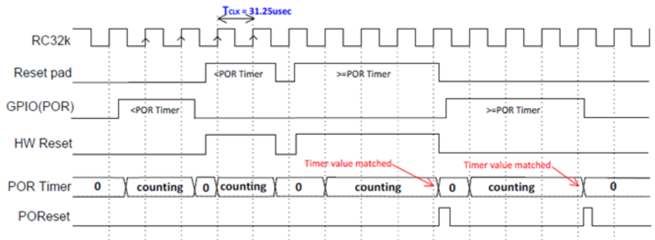
Figure 6 Power-On Reset Timing Diagram
