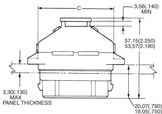
With Flange Endbell (Plug Only)
