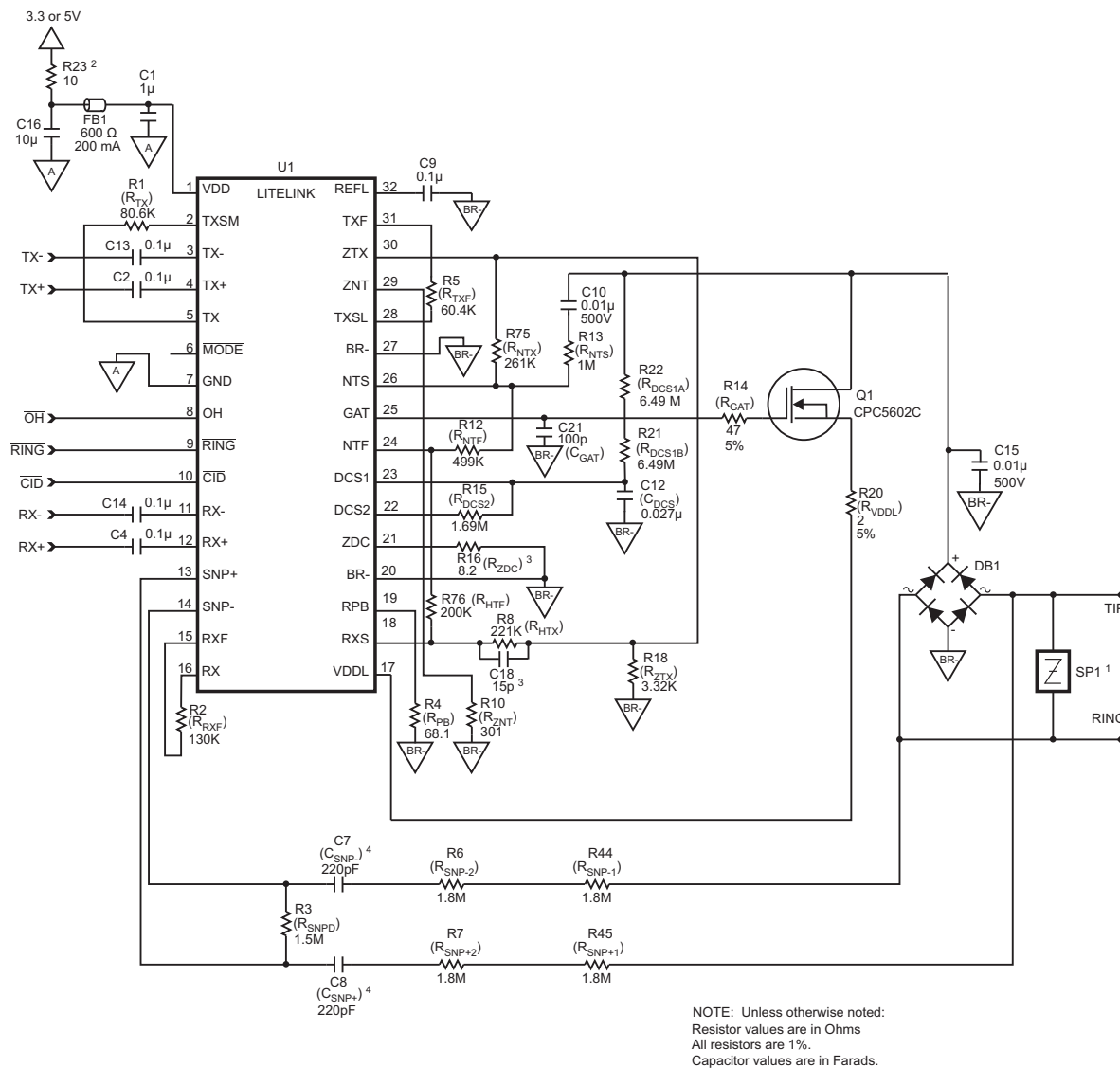
Figure 3. Resistive Termination Application Circuit Schematic
