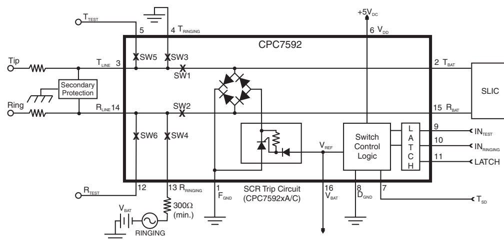
Figure 1. CPC7592 Block Diagram
