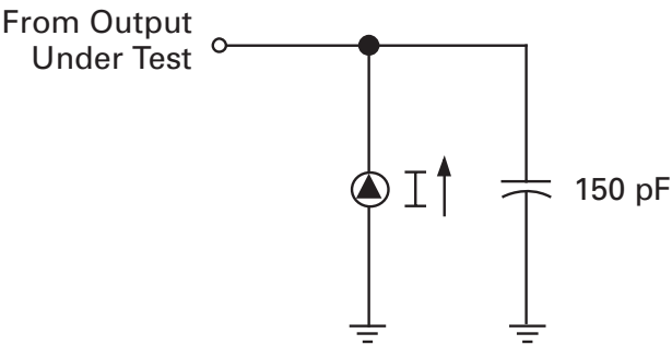
Figure 7. Test Load Diagram
