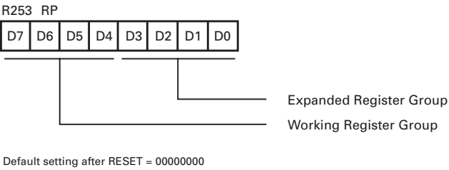
Figure 20. Register Pointer
