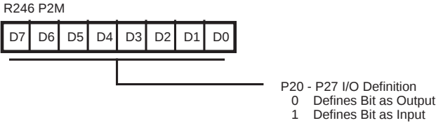
Figure 46. Port 2 Mode Register (F6 H : WRITE ONLY)
