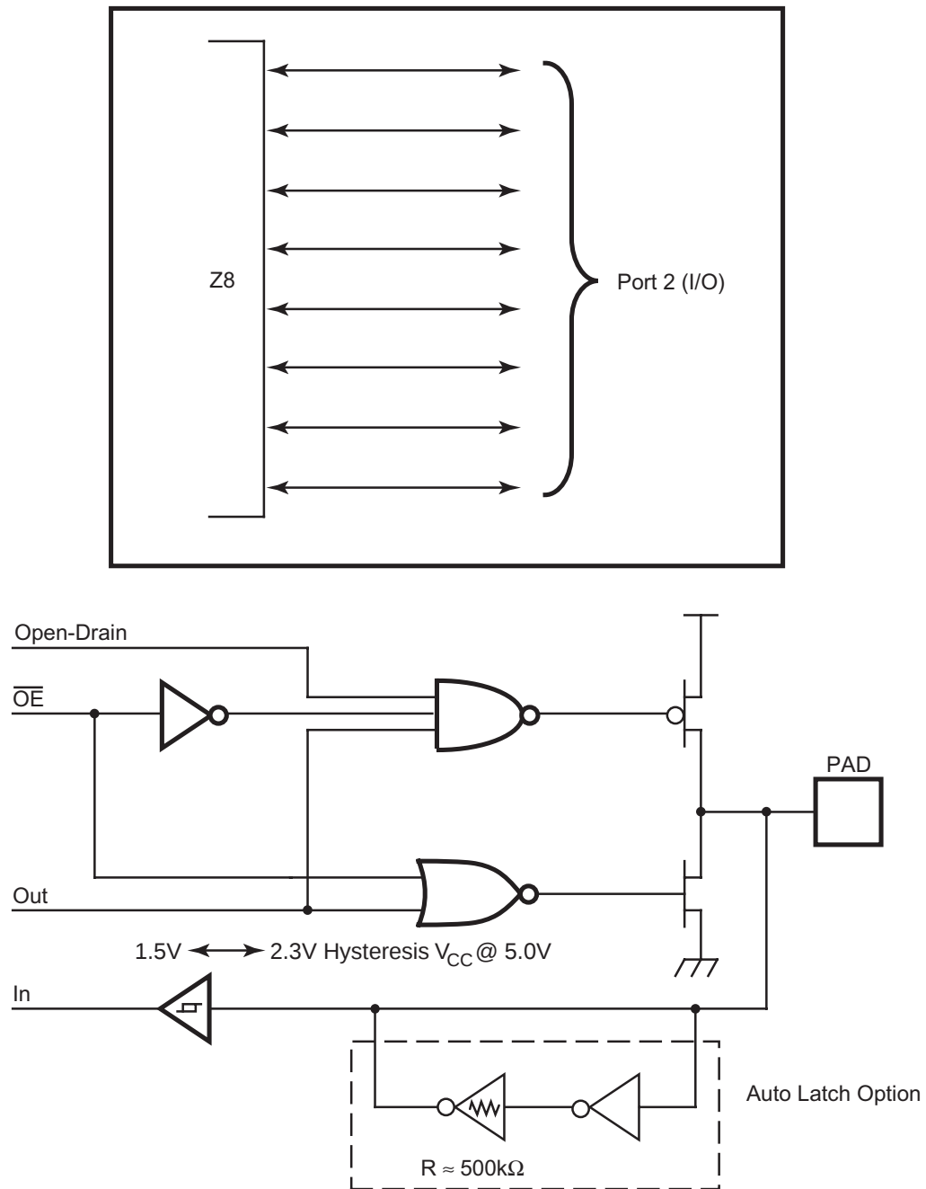
Figure 10. Port 2 Configuration
