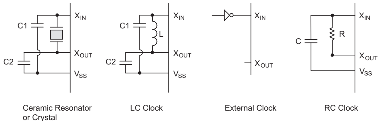
Figure 18. Oscillator Configuration
