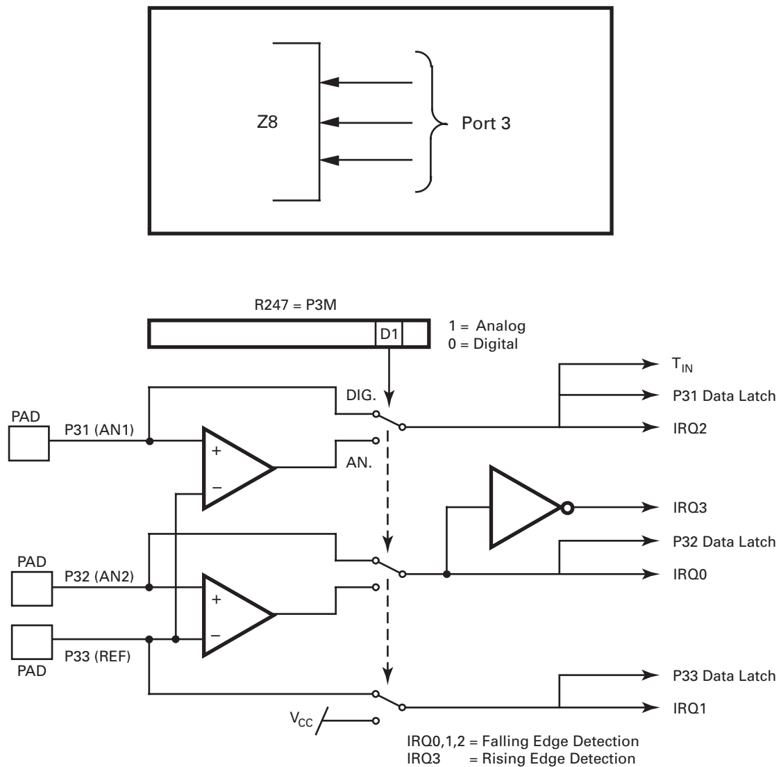
Figure 11. Port 3 Configuration
