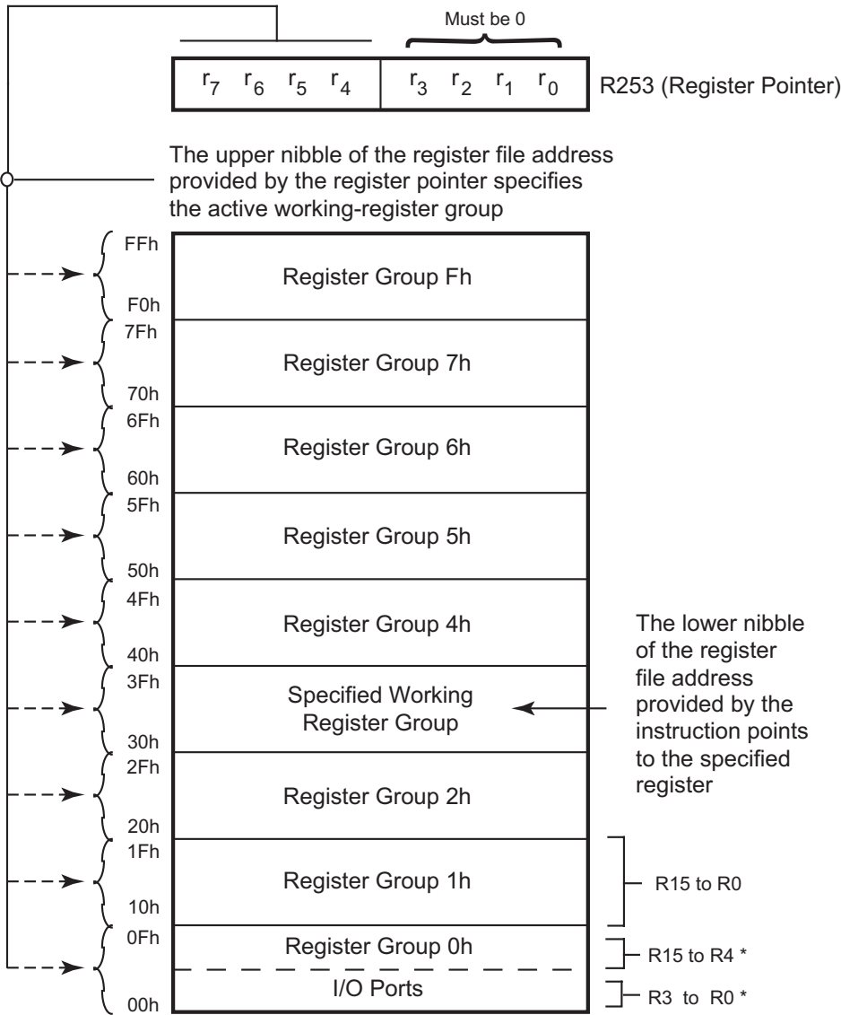
Figure 15. Register Pointer
