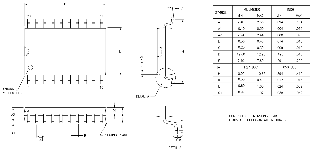
Figure 22. 20-Pin SSOP Package Diagram
