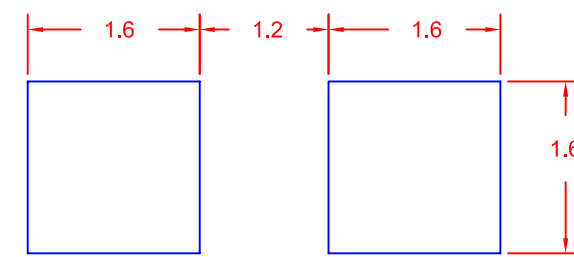
RECOMMENDED SOLDERING PAD LAYOUT
