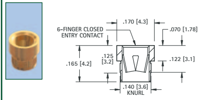
.084 (2.13) - .102 (2.6) PIN - PRESS-FIT
