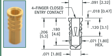
.032 (.56) - .046 (1.17) PIN - PRESS-FIT
