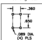
Mounting Detail For Two Holders
