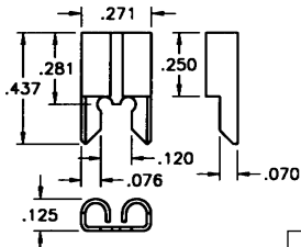
Mounting Detail For Two Clips
