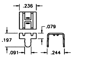
Mounting Detail For Two Clips
