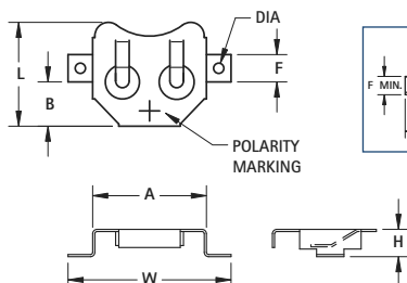
Mounting Detail
