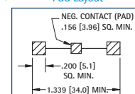
Pad Layout
