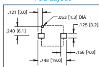
Pad Layout
