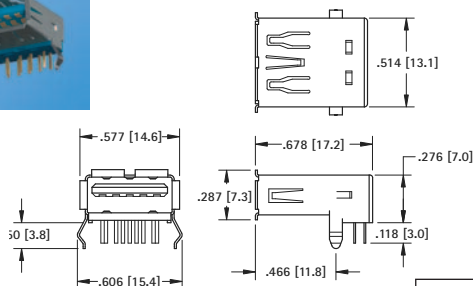
THRU-HOLE MOUNT SOCKET
