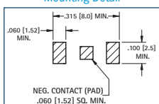
Mounting Detail
