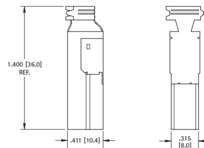
CABLE PLUG
