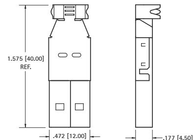
CABLE PLUG
