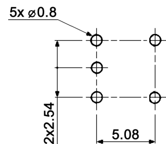
P.C. MOUNTING
