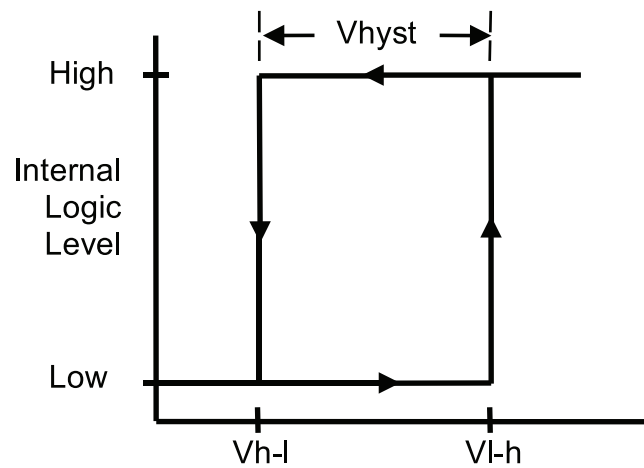
Figure 1: Hysteresis Diagram
