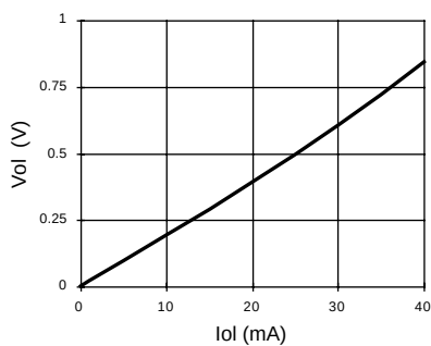
Vol vs Iol
