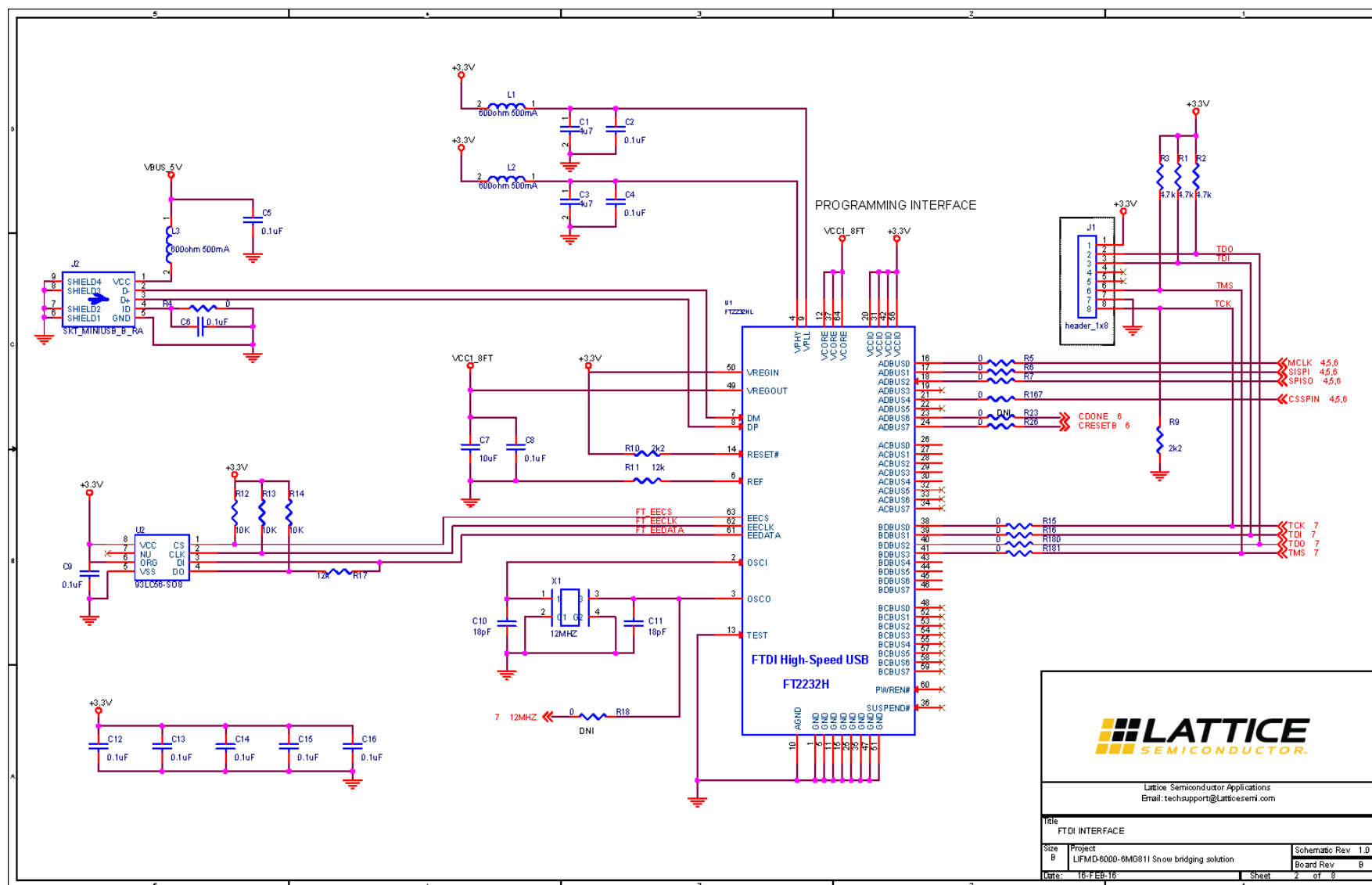
FTDI Interface
