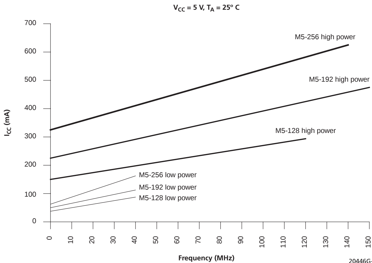
Figure 9. I_{CC} Curves at High/Low Power Modes
