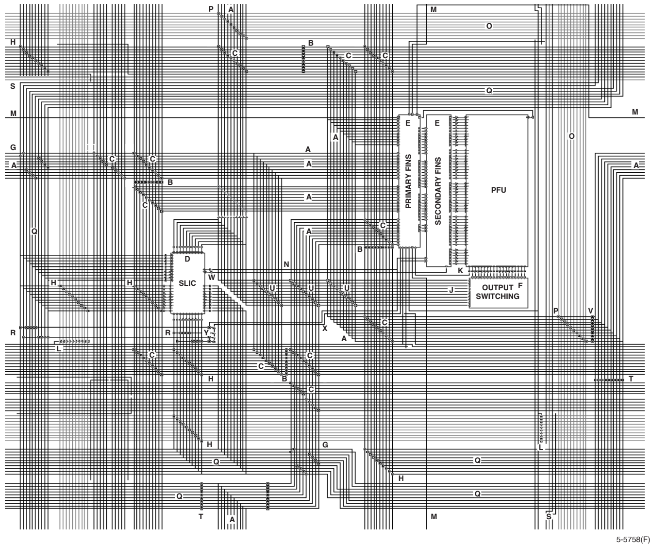
Figure 21. PLC Architecture
