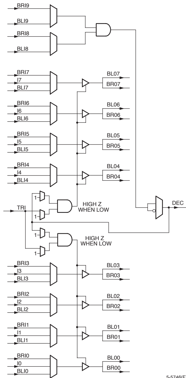
Figure 13. Buffer-Buffer-Decoder Mode
