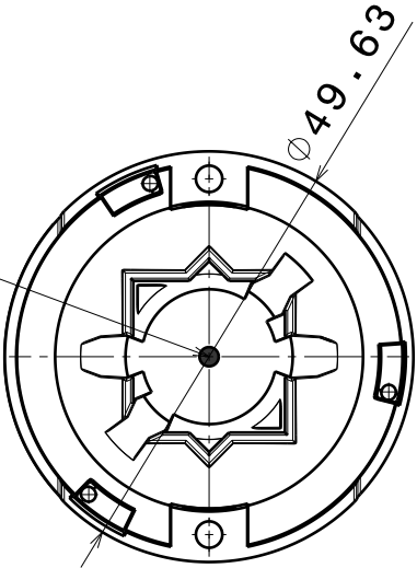
Bottom view
