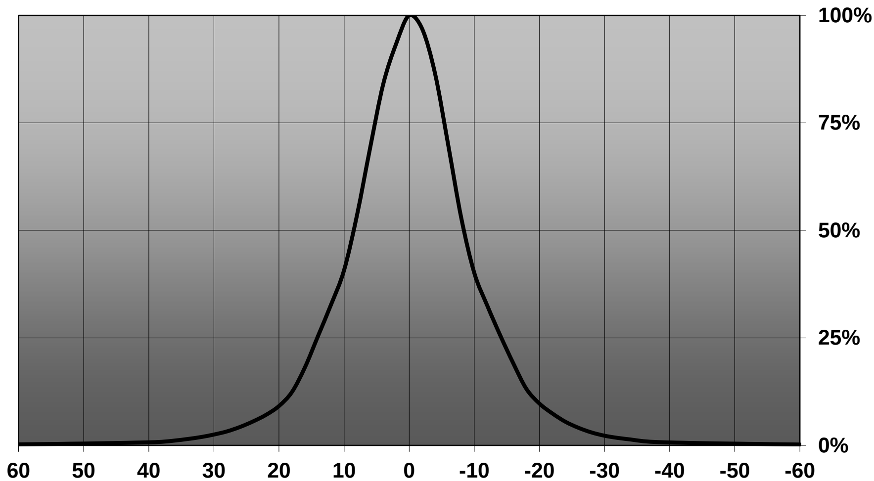
Relative intensity of FA10888_TINA-RS_(NS6x83)
