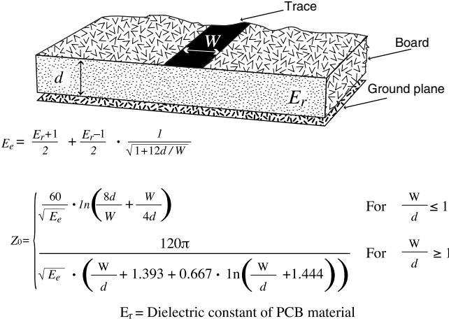
Figure 77: Microstrip Formulas
