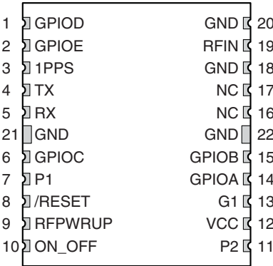
Figure 5: F4 Series GPS Receiver Pinout (Top View)
