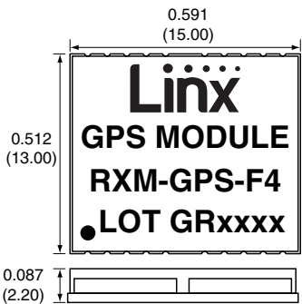
Figure 1: Package Dimensions
