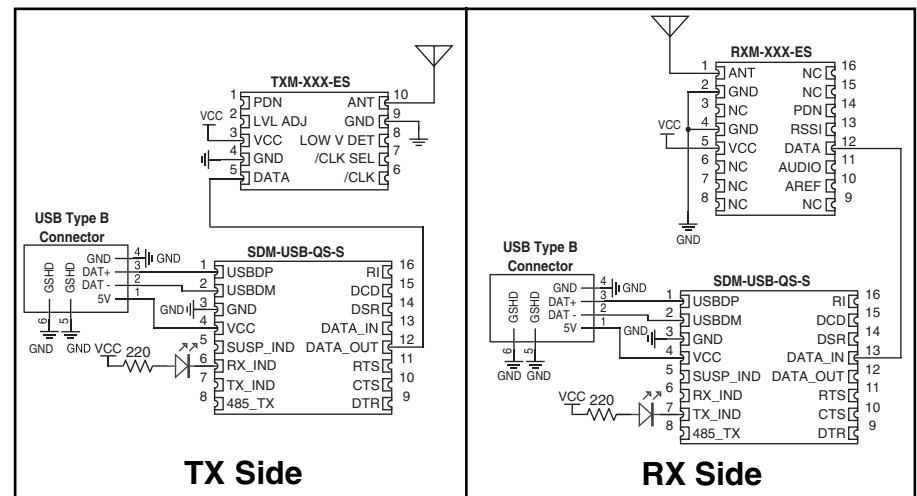
Figure 10: Wireless Modem Using The Linx ES Series RF Modules
