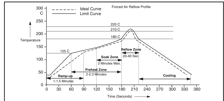
Figure 5: Maximum Reflow Profile
