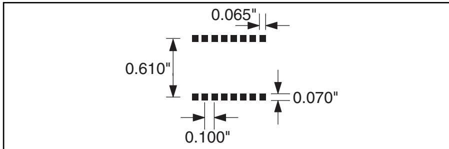
Figure 3: Recommended PCB Layout
