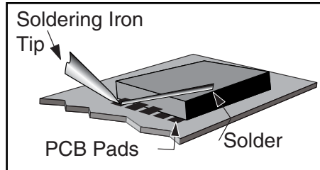
Figure 4: QS Soldering Technique
