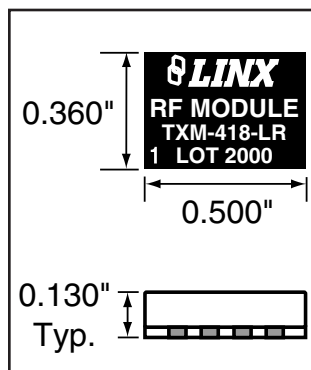
Figure 1: Package Dimensions
